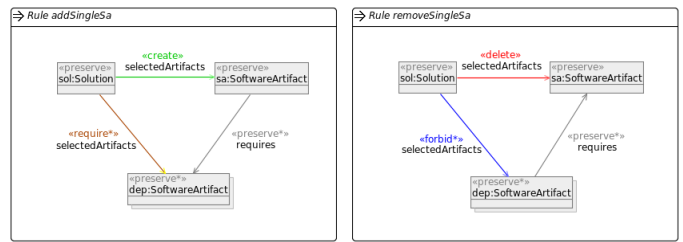
Fig. 3: Mutation rules for NRP [8]
