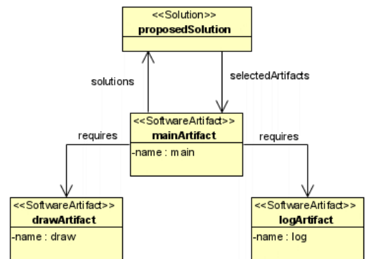
Fig. 4: Simple NRP instance
