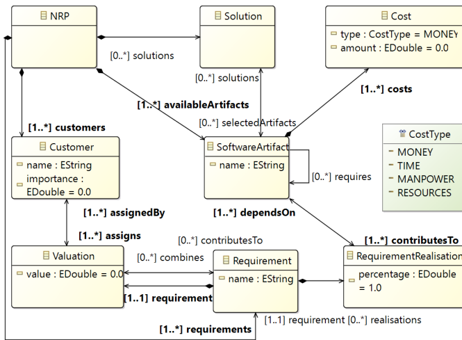
Fig. 2: Meta model for NRP [8]
